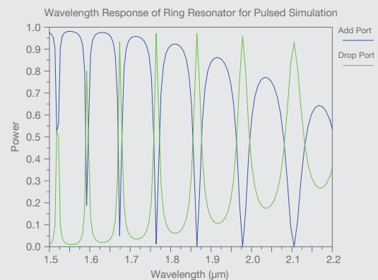
Top: CW response of ring resonator run at a wavelength resonance of 1.593μm
