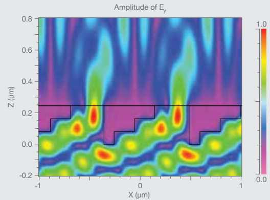
Field profile of metallic grating structure
