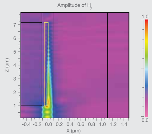
Simulated field within a surface plasmon based interferometer that is operating out of phase
