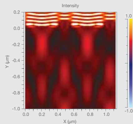
Simulation of a Phase Shift Mask with DiffractMOD
