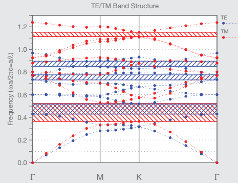
Band structure for a 2D hexagonal lattice of air holes
